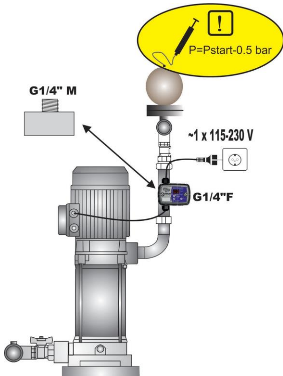
SWITCHMATIC 1/2
